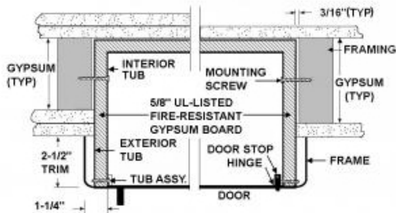
TYPICAL FIRE-RATED INSTALLATION
